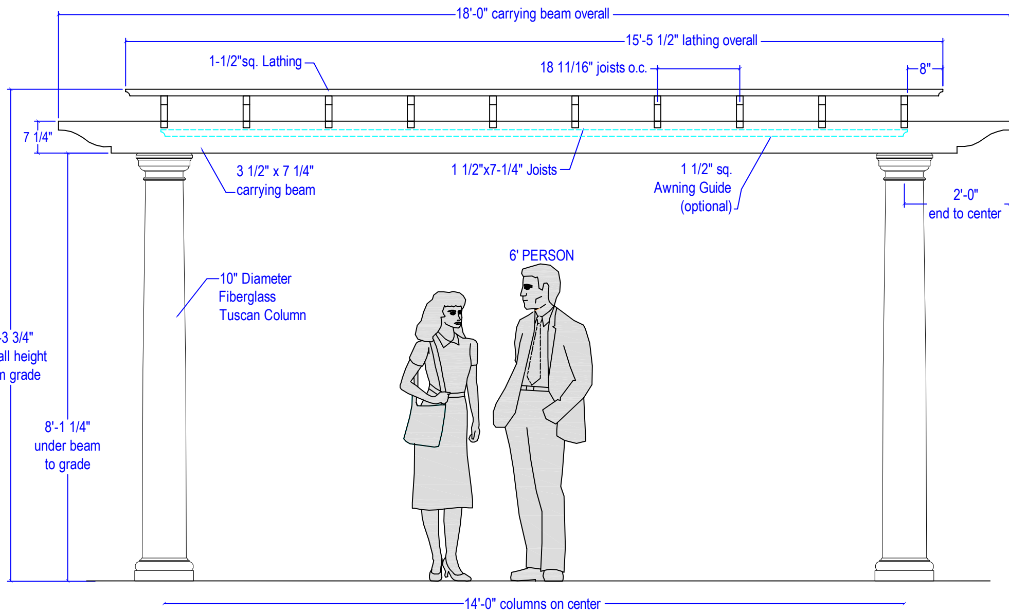
1 10x14 & 12x14 Side View (Flat) not to scale
