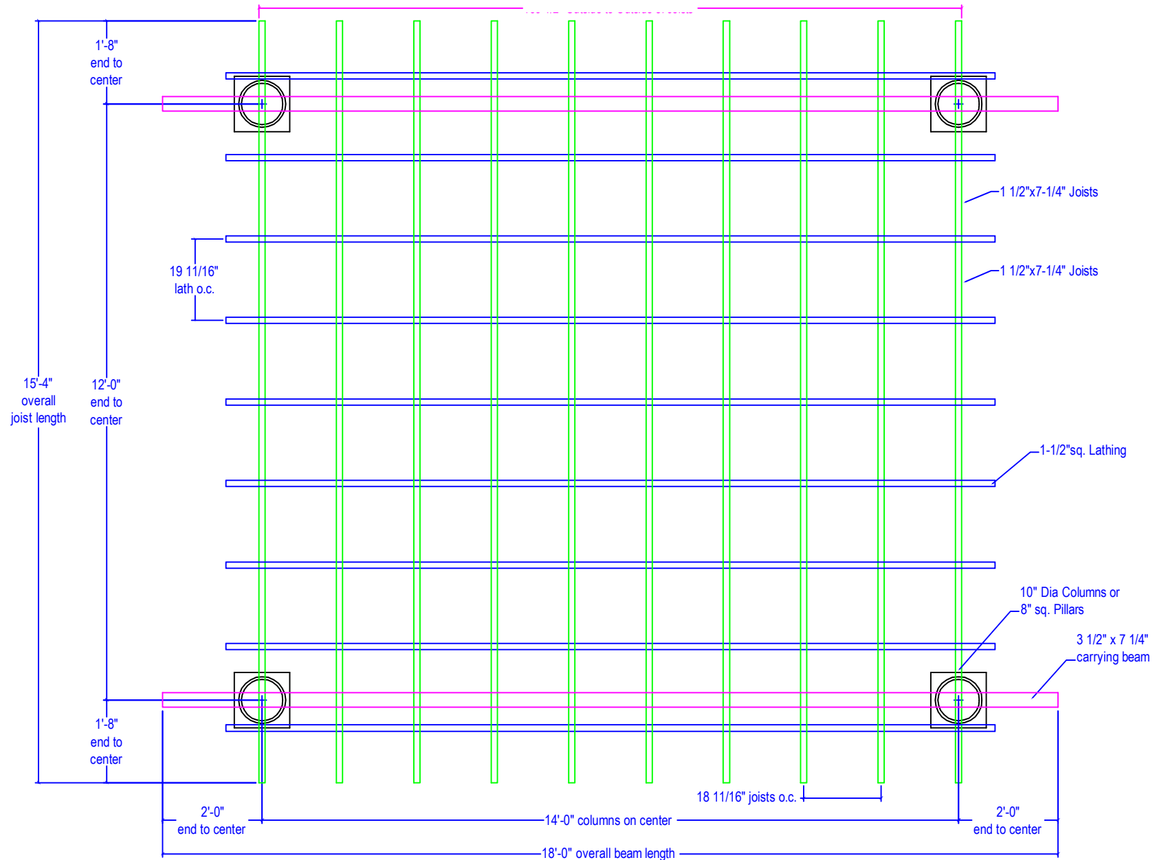
1 12x14 Plan View Flat Top SKU# 795389 not to scale
