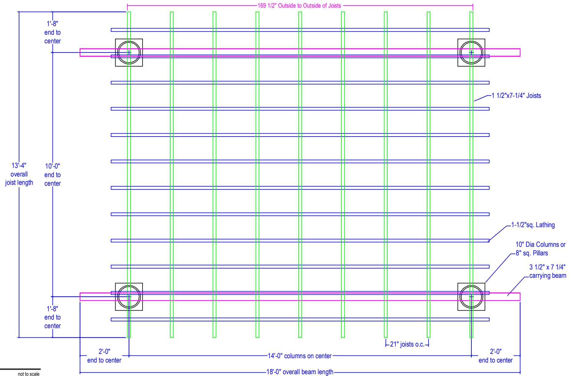
1 10x14 Plan View Arched Top SKU# 795392
